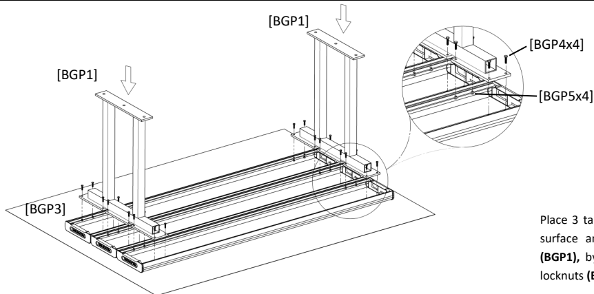
BOLT DOWN PARK SETTING (CODE No. FELAGPS)
