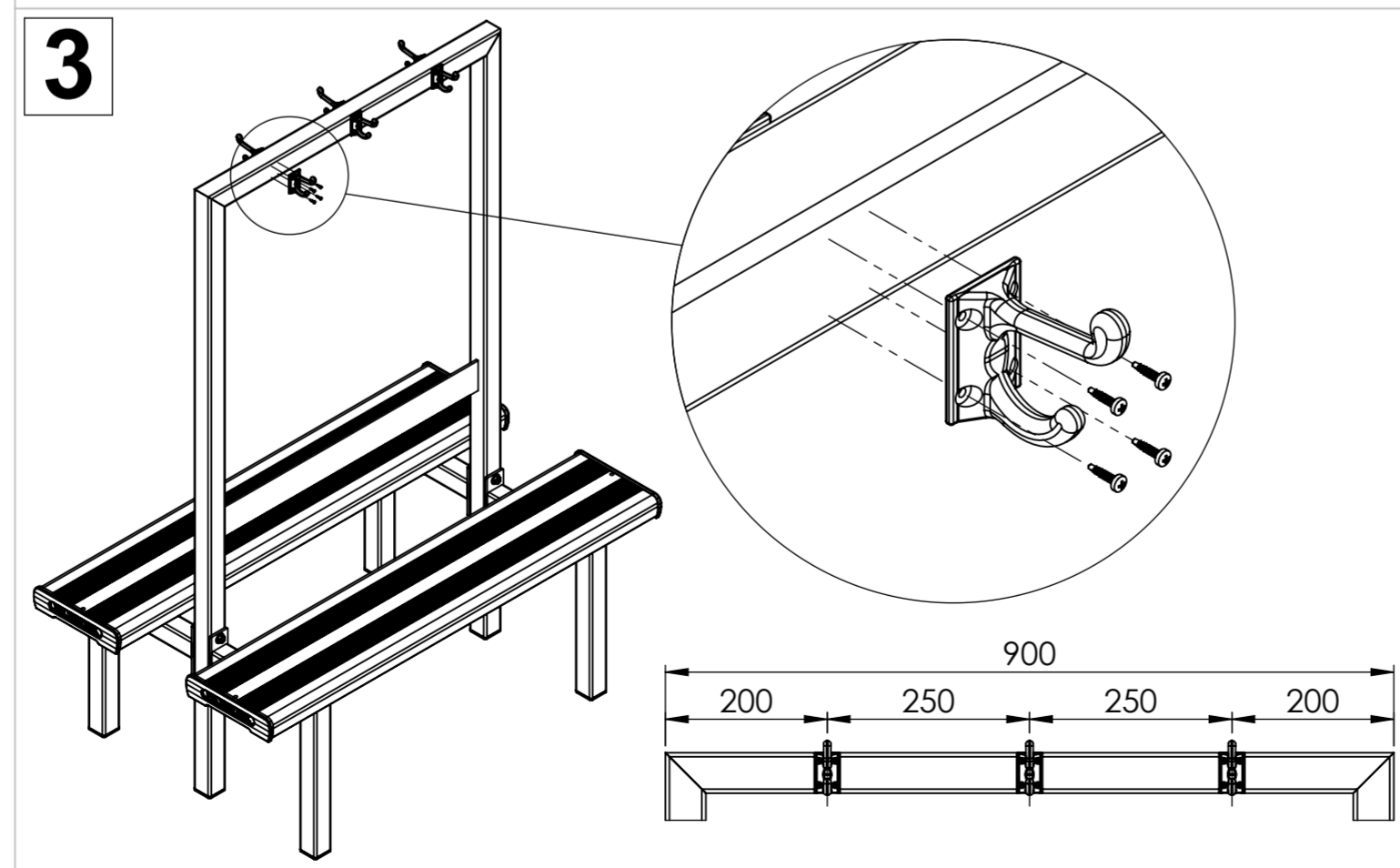
Attach six coat hooks (4) to the top bar of the frame by using self-tapping screws (10) as illustrated
