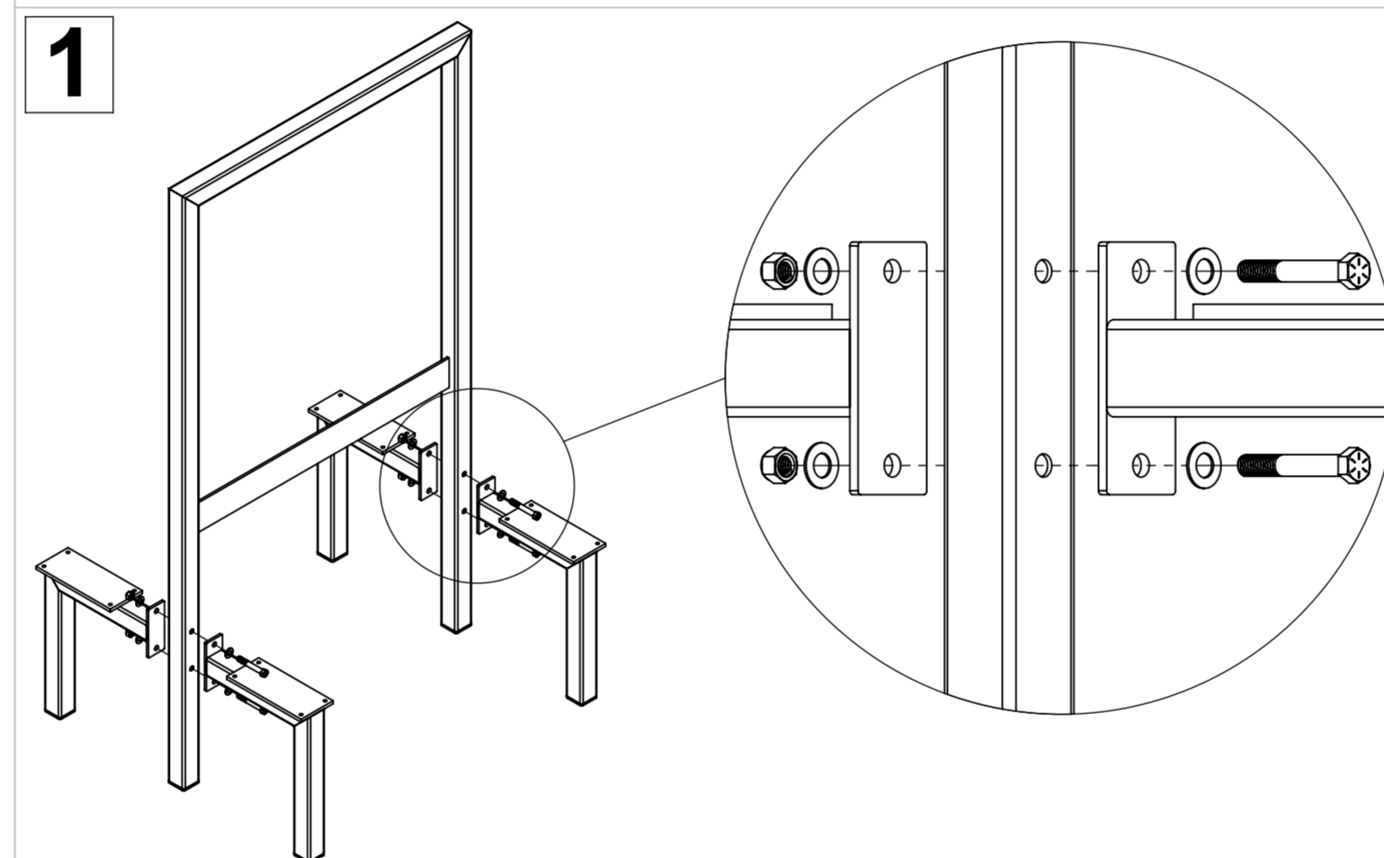
Attach four seat frames (2) to the main frame (1) by using bolts (5), washers (6) and nuts (7) as illustrated
