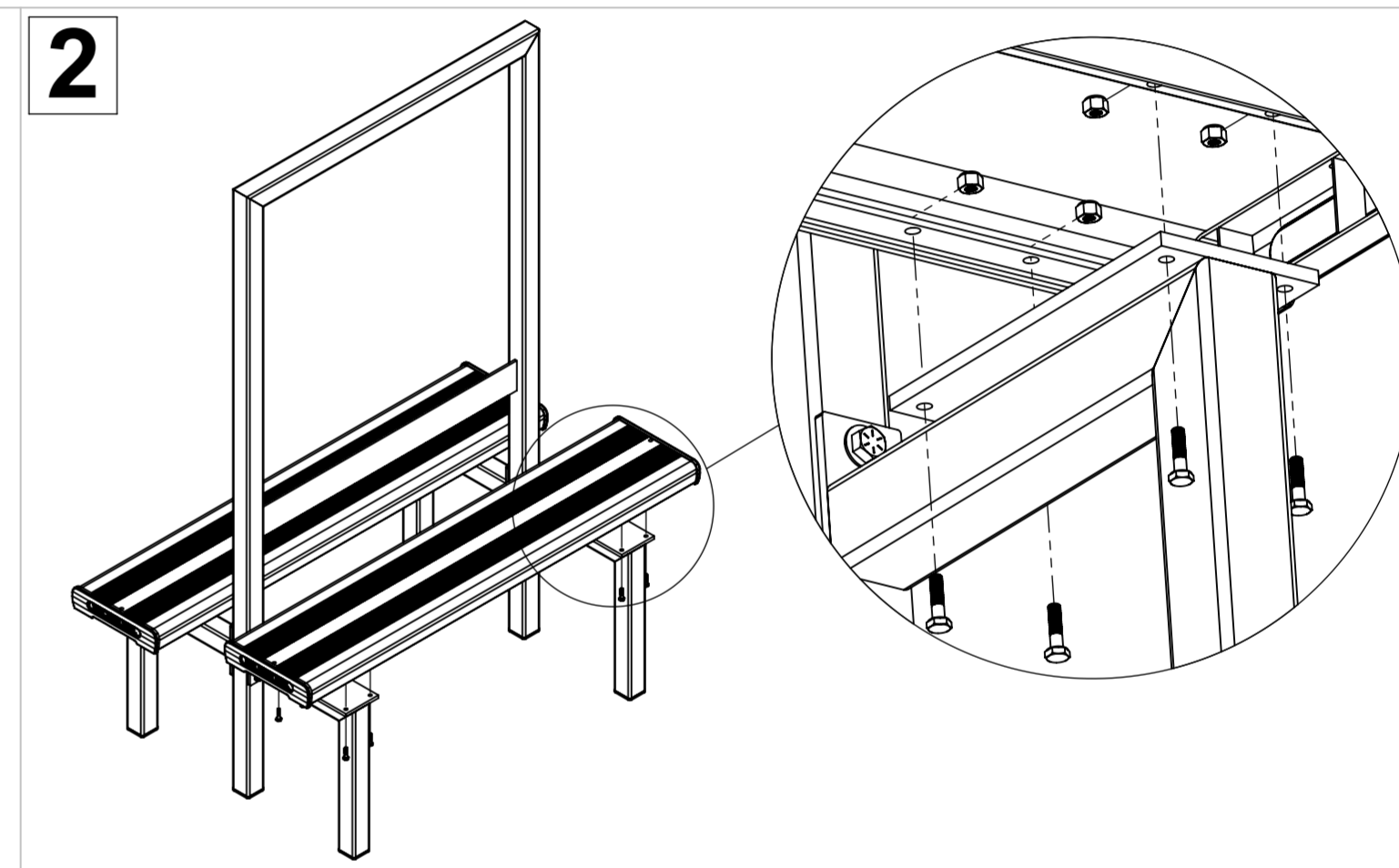
Attach two seat planks (3) to the assembly in step 1 by using bolts (8) and nuts (9) as illustrated
